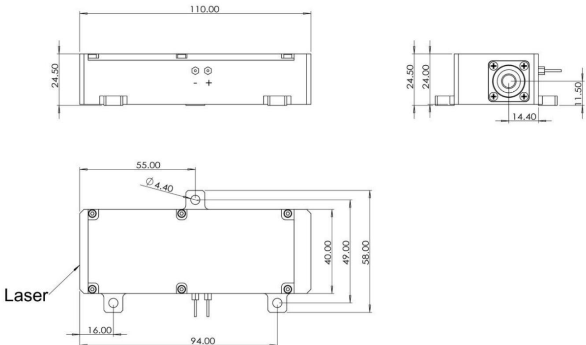
Figure 2 ER8000 / ER10000 Outline Dimensions
