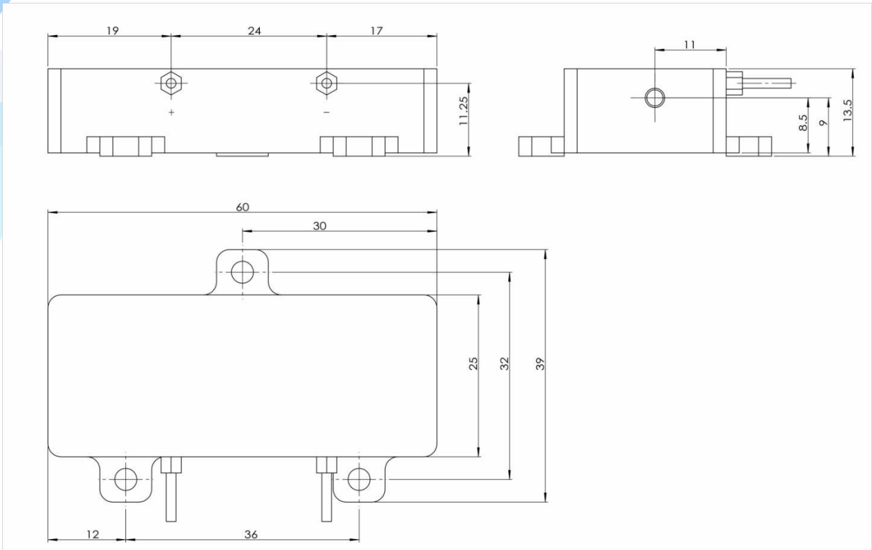
Figure 1 ER2000 / ER4000 Outline Dimensions
