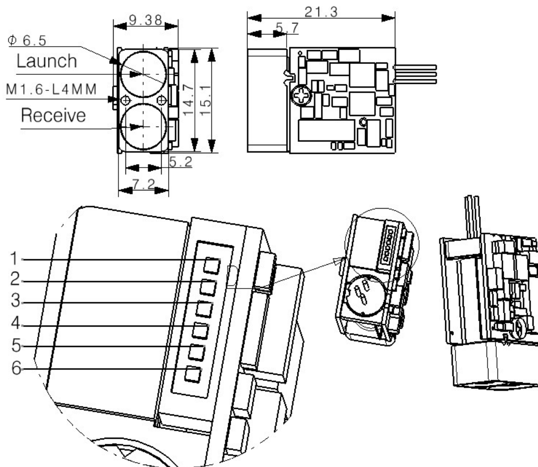
SPD1200N2 source mechanical and pin-callout figure — model-specific dimensions and 1–6 pin order retained; not for manufacturing.
