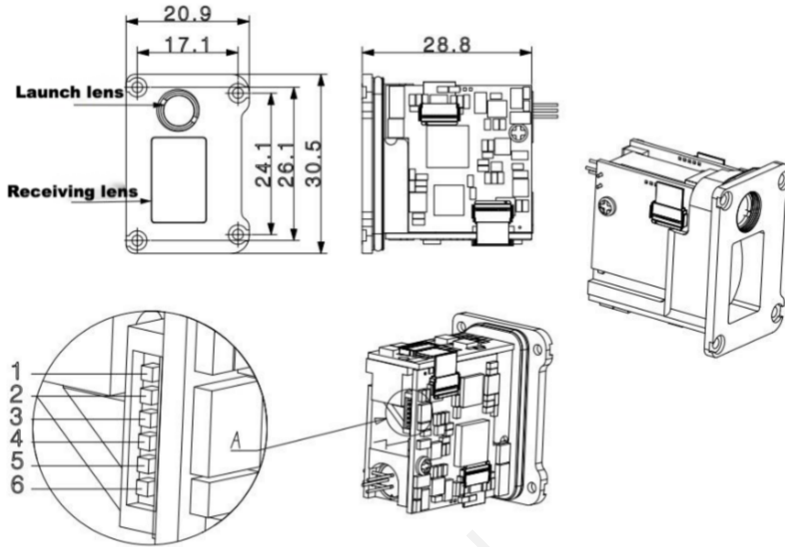
Mechanical Dimension Drawing and Electrical Interface Diagram
