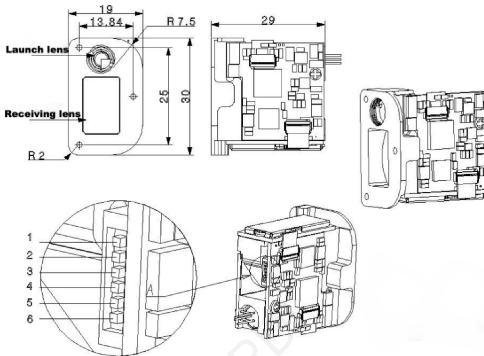
Mechanical Dimension Drawing and Electrical Interface Diagram
