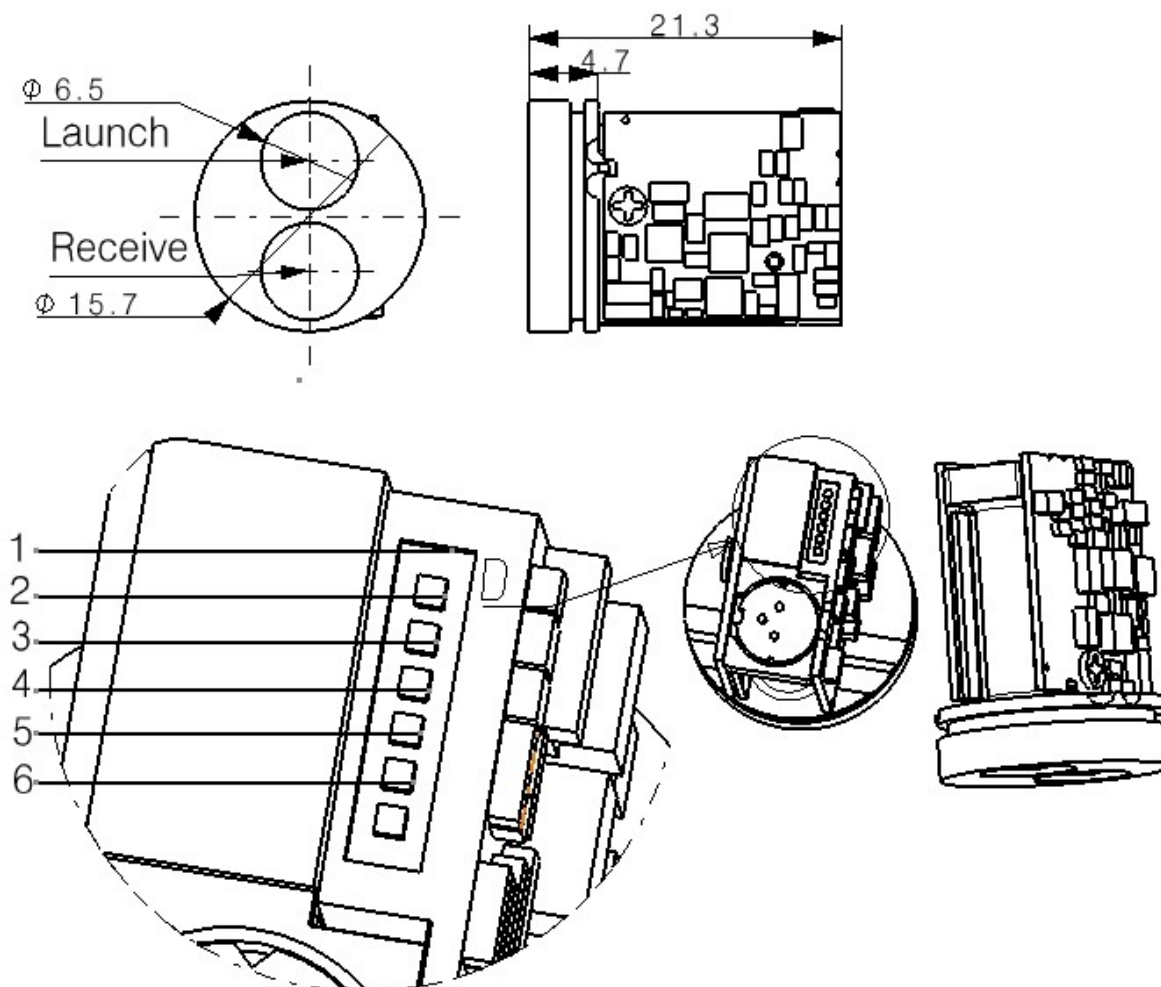
SPD1200N0 source mechanical and pin-callout figure — model-specific dimensions retained; not for manufacturing.
