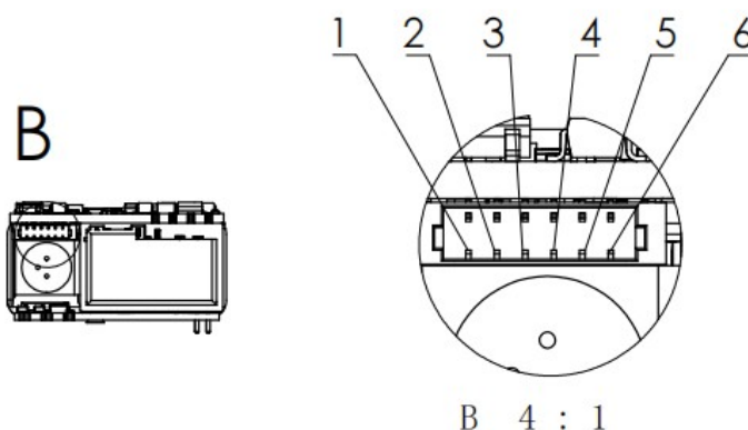
6-Pin Connector and Pin Assignments
